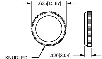
PLASTIC FACENUT
