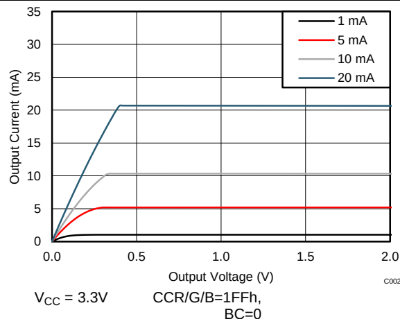
Figure 2. Output Current vs Output Voltage
