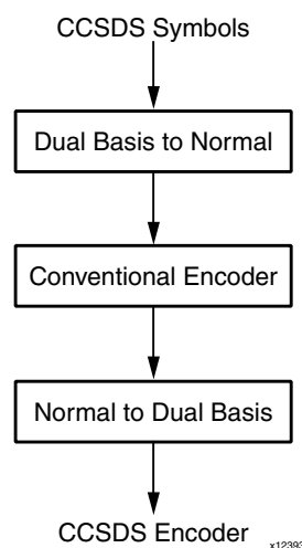
Figure 4-1: CCSDS Encoder
