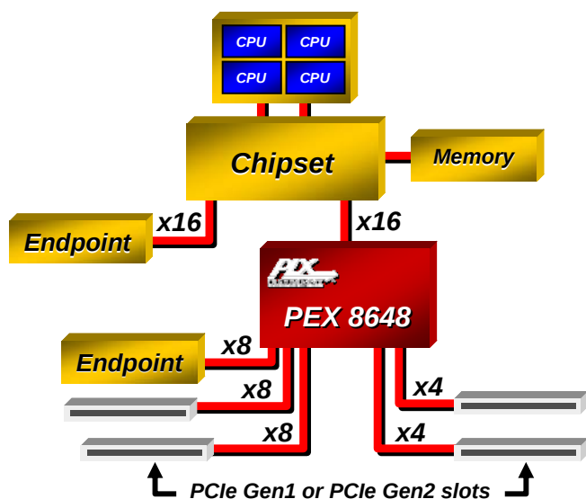
Figure 3. Fan-in/out Usage
