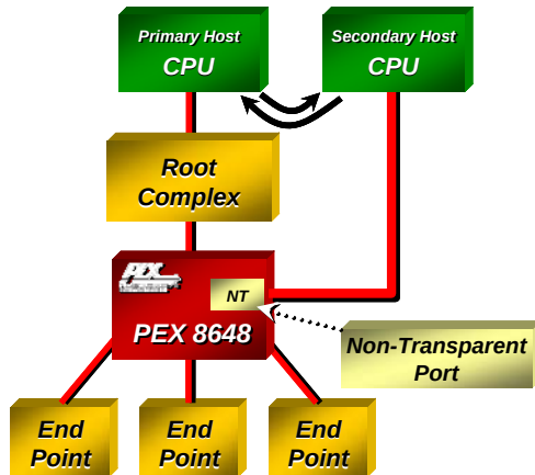
Figure 2. Non-Transparent Port
