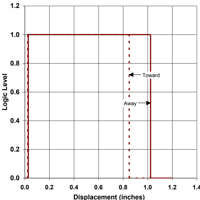
Typical - Voltage vs Displacement Avery Label 5160
