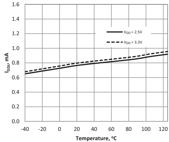
Figure 4: Typical Logic Low Output Supply Current I_{DDL} vs. Temperature
