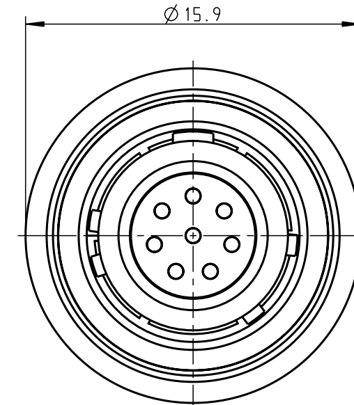
S11YAR-P08XFG0-0000 Mechanical coding: A Color coding: light brown
