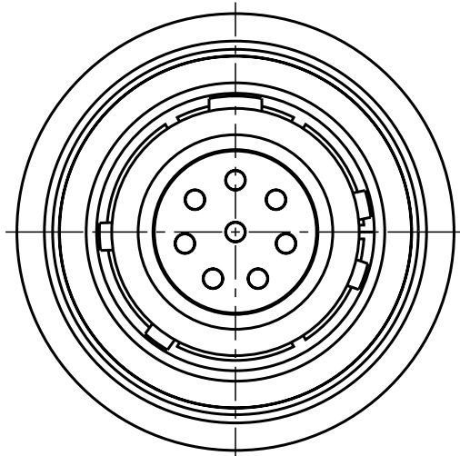
S11YBR-P08XFG0-0000 Mechanical coding: B Color coding: red
