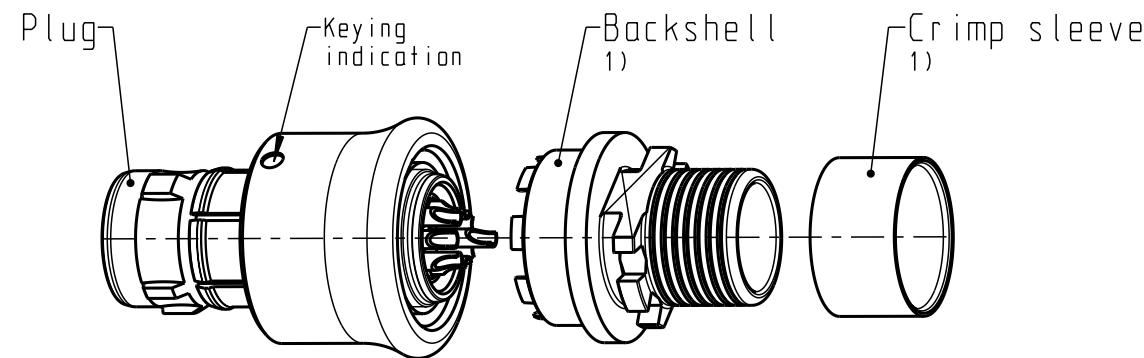
Delivery condition 2:1
