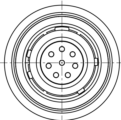
S11YCR-P08XFG0-0000 Mechanical coding: C Color coding: blue
