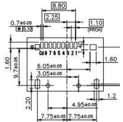
Recommend PC Board layout
