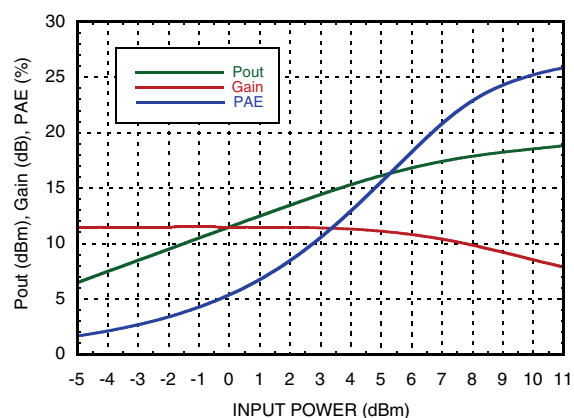
Pout, Gain & PAE @ 2 GHz
