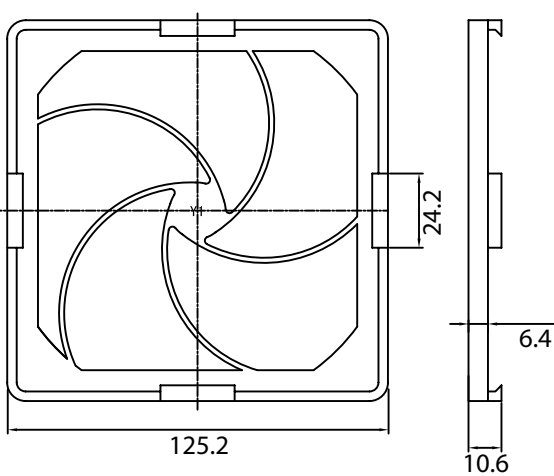
RETAINER
