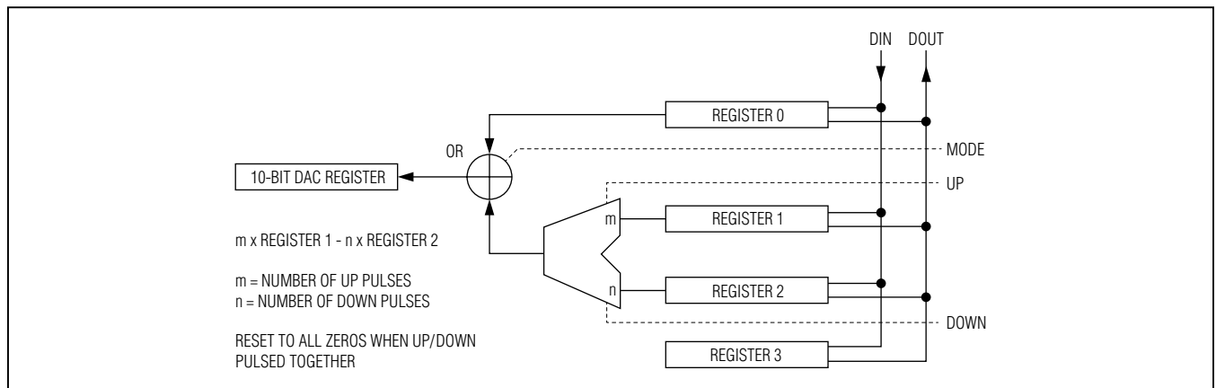
Figure 1. Register Configuration Diagram
