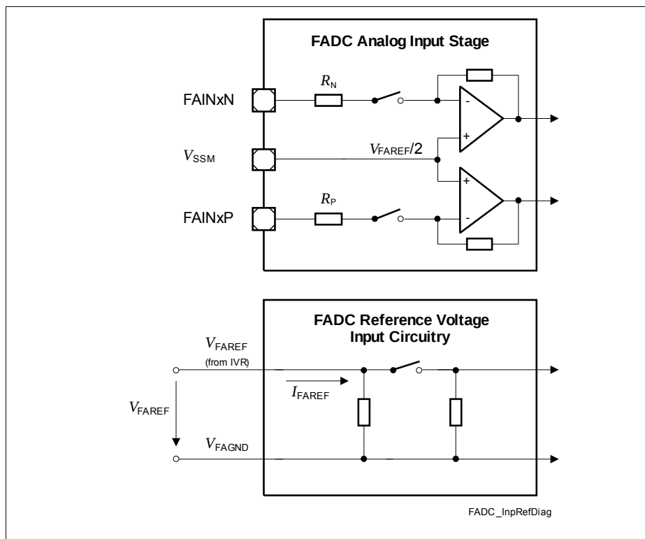
Figure 5 FADC Input Circuits
