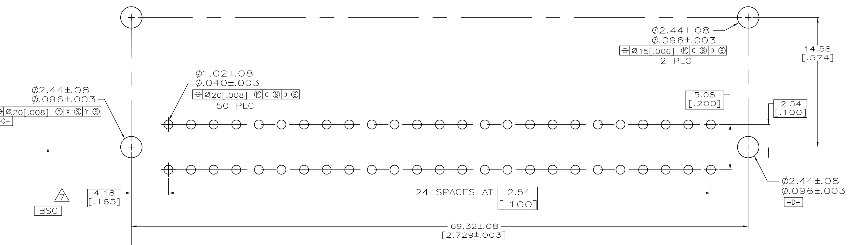
RECOMMENDED PC BOARD HOLE LAYOUT
