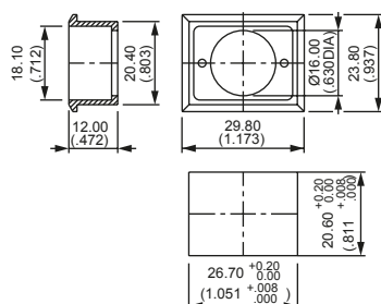
Rectangular : A01FM1
