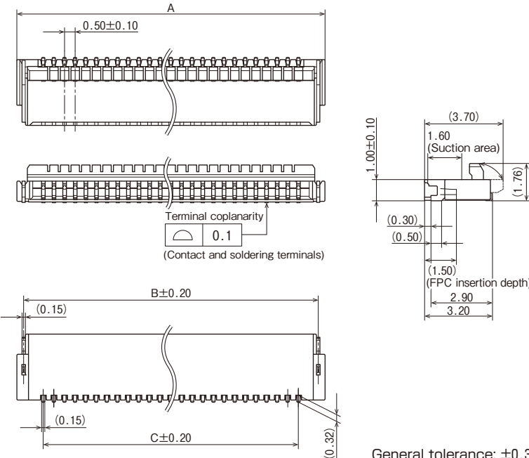
External dimensions
