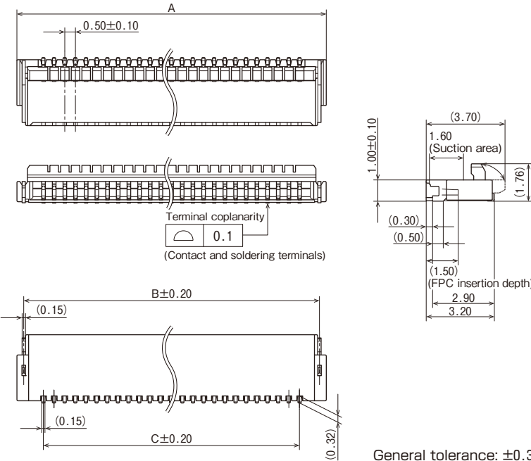
External dimensions
