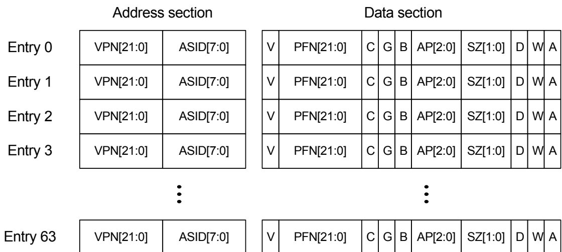
Figure 5-5. TLB organization
