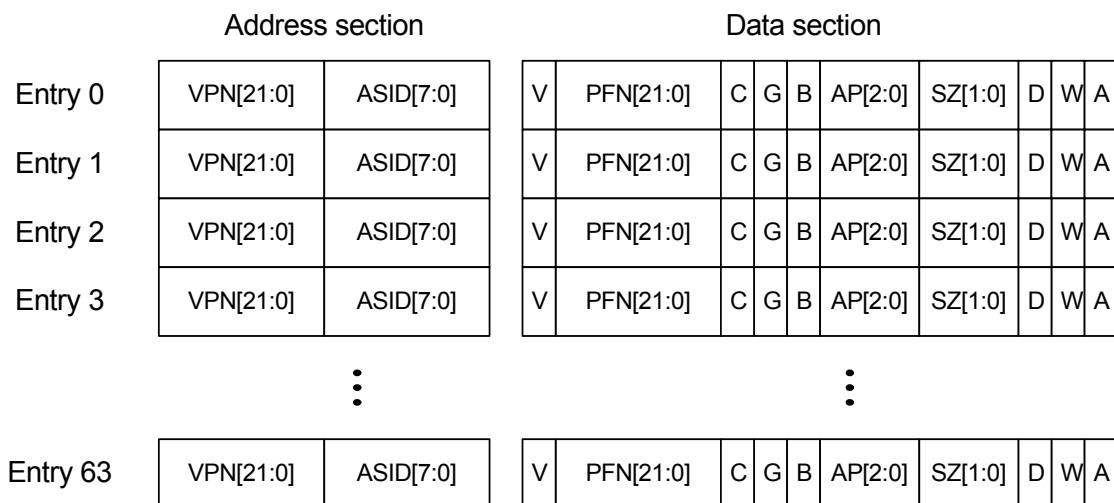
Figure 5-5. TLB organization
