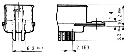
Solder cup type
