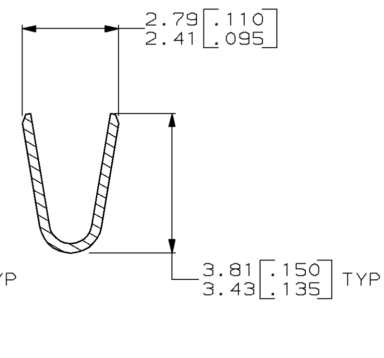
SECTION C-C
