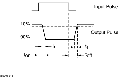
Fig. 2 - Switching Times Measurement Test Circuit and Waveform
