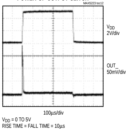
POWER-UP OUTPUT GLITCH
