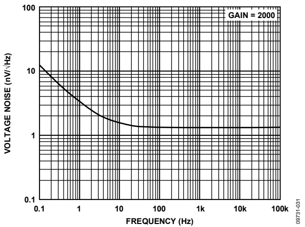
Figure 29. RTI Voltage Noise Spectral Density vs. Frequency
