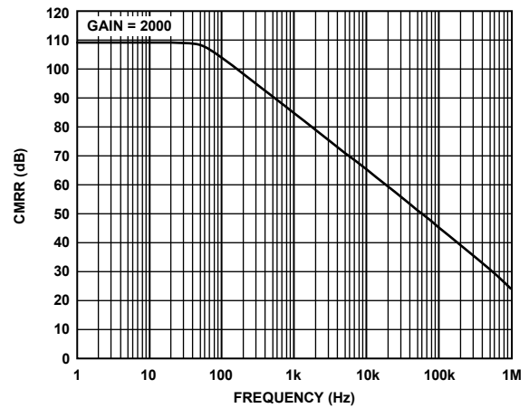
Figure 14. CMRR vs. Frequency, 1 kΩ Source Imbalance
