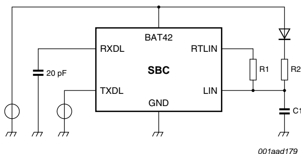
Fig 27. Timing test circuit for LIN transceiver
