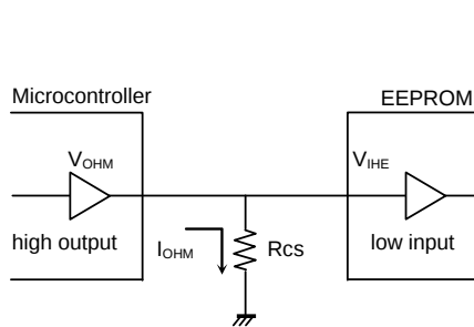
Figure 44. CS pull down resistance
