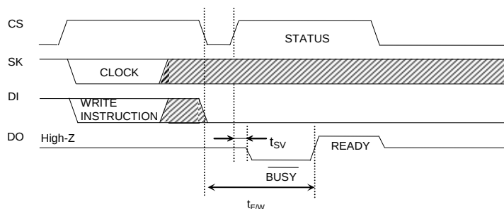
Figure 48. READY/ \overline{BUSY} STATUS output timing chart
