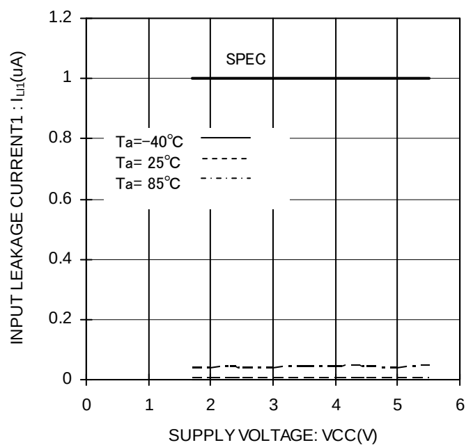
Figure 11. Input leakage current1 I_{LI1} (SK)
