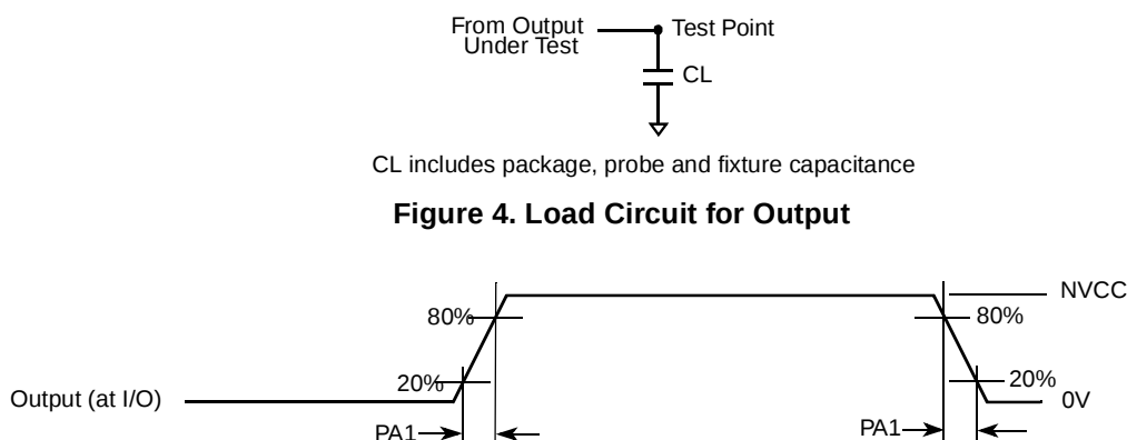
Figure 5. Output Transition Time Waveform
