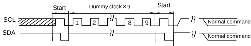
Figure 45-(b). The Case of START + Dummy Clock \times 9 + START + Command Input
