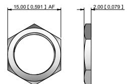
M12 x 0.75 THREAD
