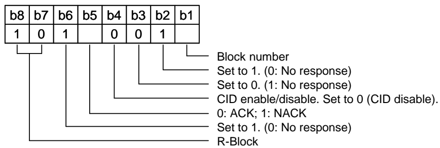
Figure 4-6 R-block Coding
