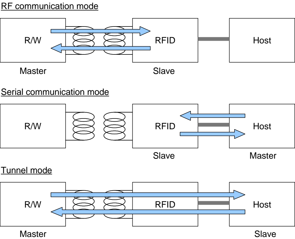
Figure 1-2 Operation Mode
