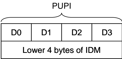
Figure 4-12 PUPI Format
