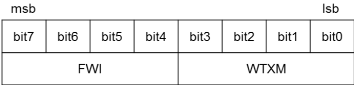
Figure 4-13 FWI Format
