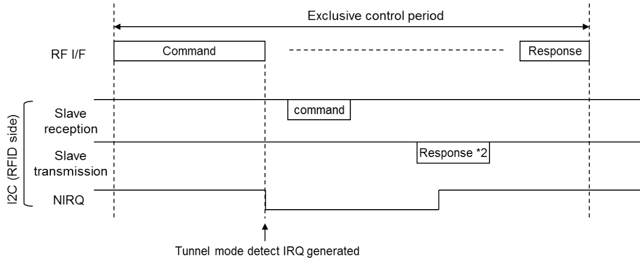
Figure 8-2 Exclusive Control in Tunnel Mode
