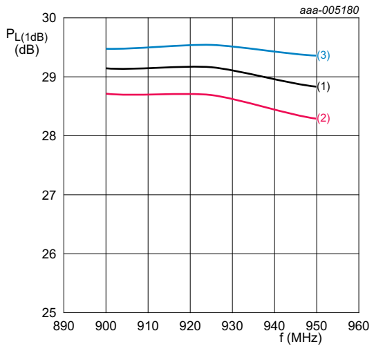
aaa-005180 V_{SUP} = 3.6\text{ V} ; I_{CC(tot)} = 70\text{ mA} ; matched for ISM-915. (1) T_{amb} = -40\text{ }^\circ\text{C} (2) T_{amb} = +25\text{ }^\circ\text{C} (3) T_{amb} = +85\text{ }^\circ\text{C}
