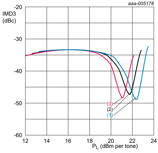
aaa-005178 V_{SUP} = 3.6\text{ V} ; I_{CC(tot)} = 70\text{ mA} ; \Delta f = 1\text{ MHz} ; matched for ISM-915. (1) T_{amb} = -40\text{ }^\circ\text{C} (2) T_{amb} = +25\text{ }^\circ\text{C} (3) T_{amb} = +85\text{ }^\circ\text{C}
