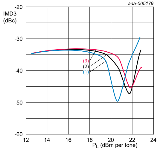
aaa-005179 T_{amb} = 25\text{ }^\circ\text{C} ; I_{CC(tot)} = 70\text{ mA} ; \Delta f = 1\text{ MHz} ; matched for ISM-915. (1) V_{SUP} = 3.3\text{ V} (2) V_{SUP} = 3.6\text{ V} (3) V_{SUP} = 3.9\text{ V}
