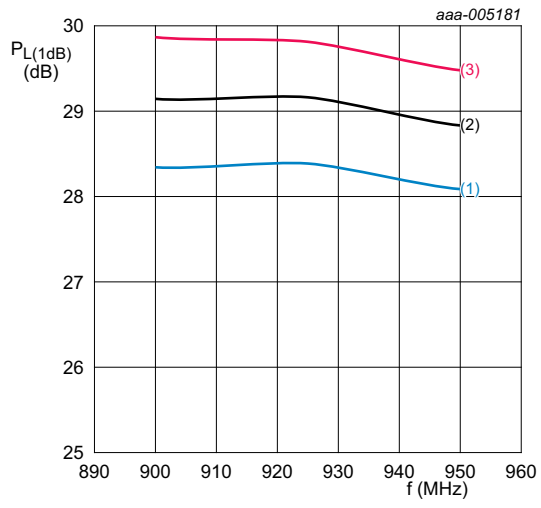
aaa-005181 T_{amb} = 25\text{ }^\circ\text{C} ; I_{CC(tot)} = 70\text{ mA} ; matched for ISM-915. (1) V_{SUP} = 3.3\text{ V} (2) V_{SUP} = 3.6\text{ V} (3) V_{SUP} = 3.9\text{ V}
