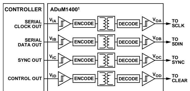
Figure 57. Isolated Interface
