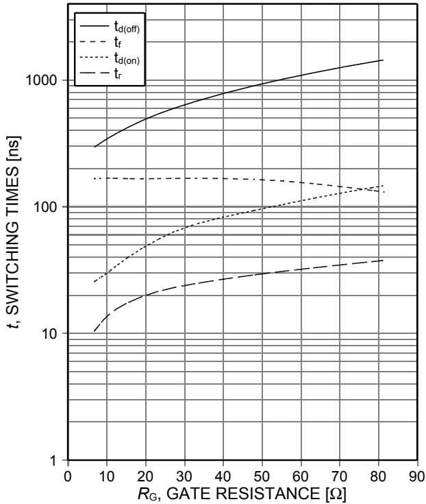
Figure 9. Typical switching times as a function of gate resistance (inductive load, T_{vj}=150^\circ\text{C} , V_{CE}=400\text{V} , V_{GE}=0/15\text{V} , I_C=30\text{A} , dynamic test circuit in Figure E)
