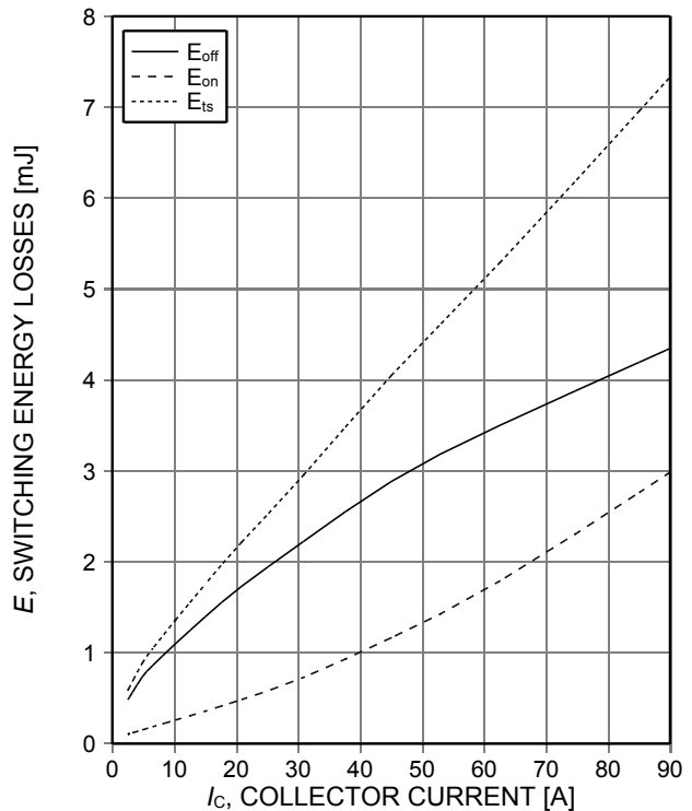
Figure 12. Typical switching energy losses as a function of collector current (inductive load, T_{vj}=150^\circ\text{C} , V_{CE}=400\text{V} , V_{GE}=0/15\text{V} , R_{G(on)}=23\Omega , R_{G(off)}=10\Omega , dynamic test circuit in Figure E)
