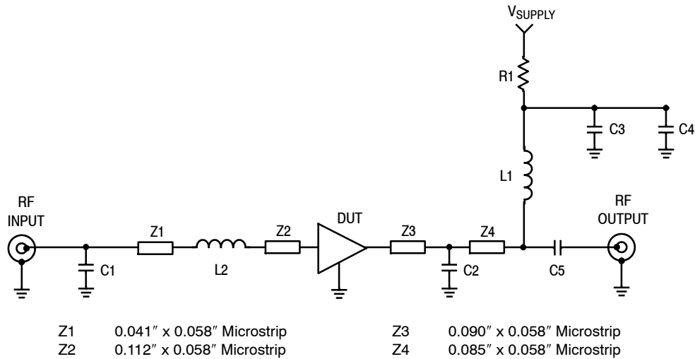
Figure 13. MMG15241HT1 Test Circuit Schematic
