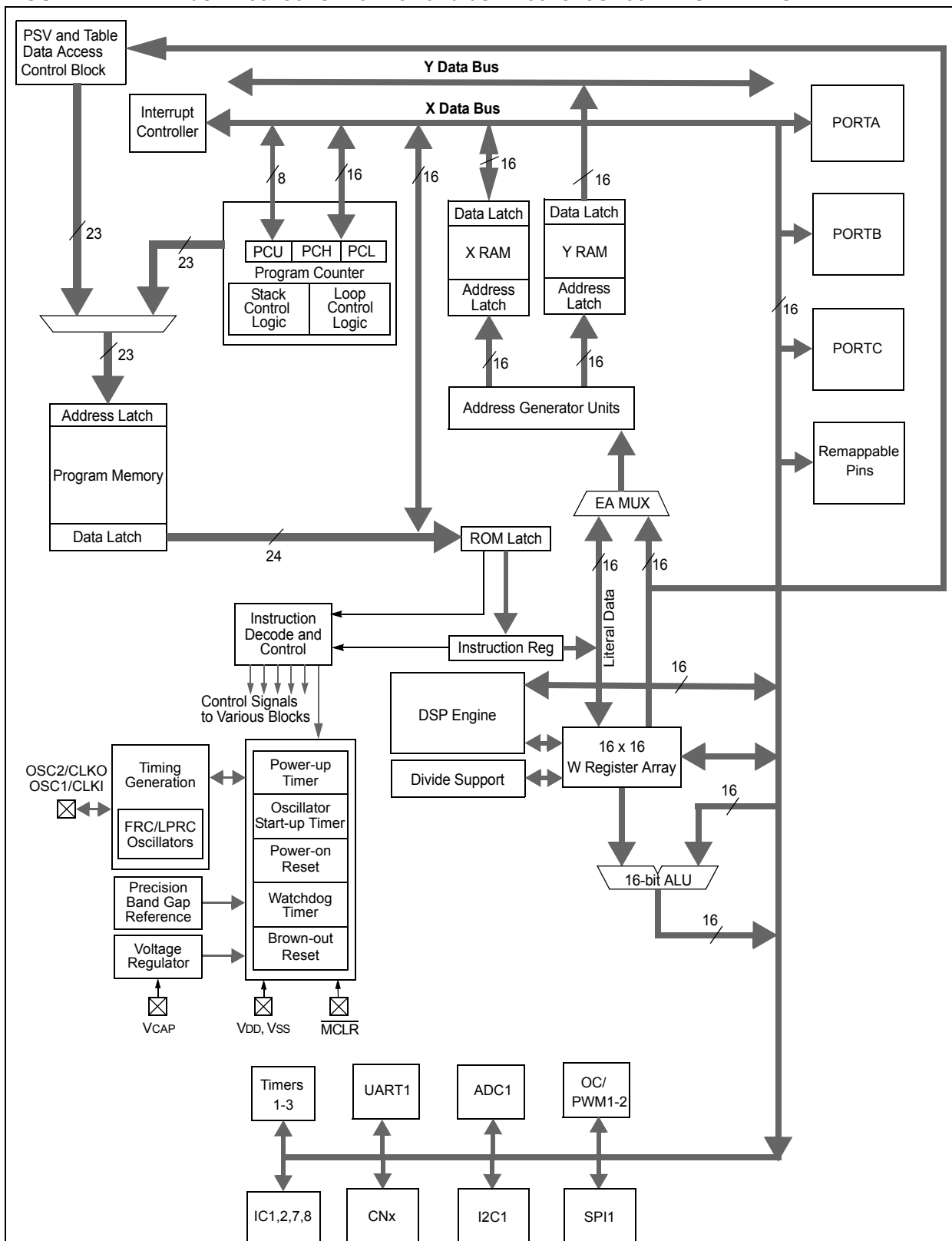
FIGURE 1-1: dsPIC33FJ32GP202/204 and dsPIC33FJ16GP304 BLOCK DIAGRAM
