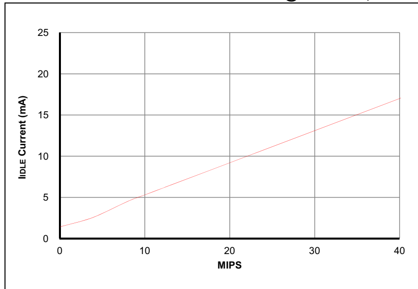
FIGURE 24-12: TYPICAL I IDLE CURRENT @ V DD = 3.3V, +85°C
