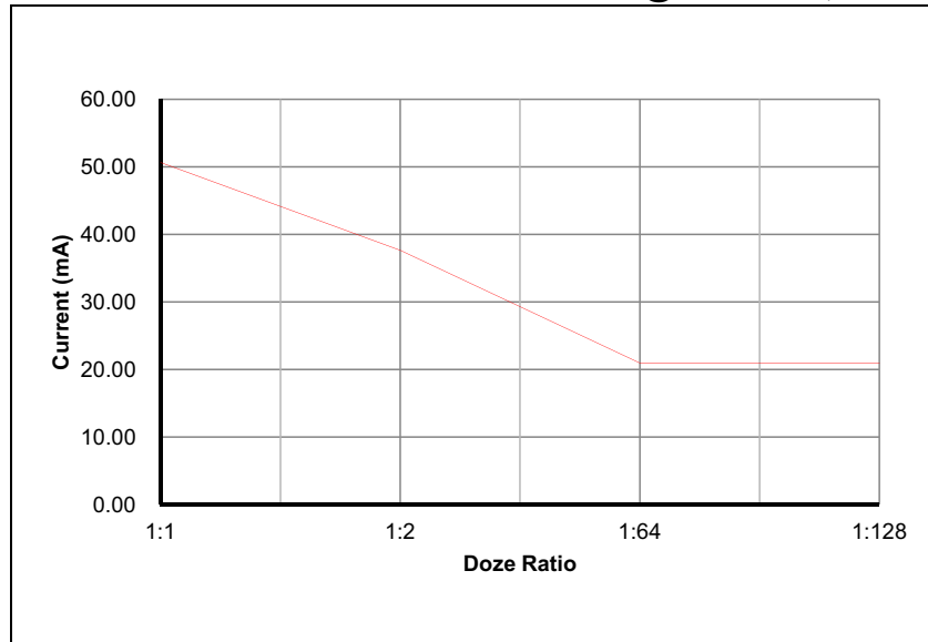
FIGURE 24-11: TYPICAL I DOZE CURRENT @ V DD = 3.3V, +85°C
