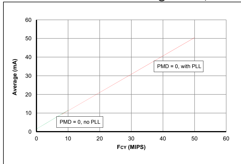
FIGURE 24-10: TYPICAL I_{DD} CURRENT @ V_{DD} = 3.3V , +85^{\circ}C
