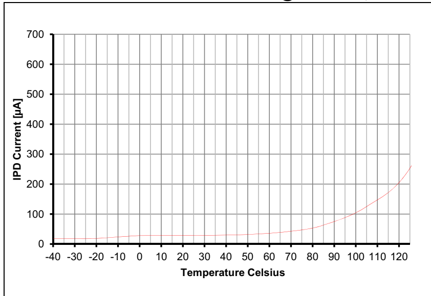
FIGURE 24-9: TYPICAL I PD CURRENT @ V DD = 3.3V, +85°C
