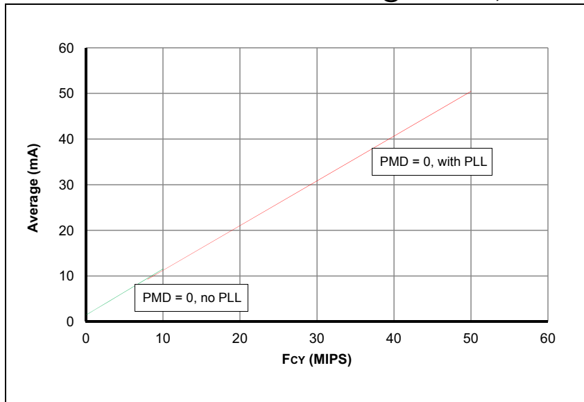
FIGURE 24-10: TYPICAL I DD CURRENT @ V DD = 3.3V, +85°C
