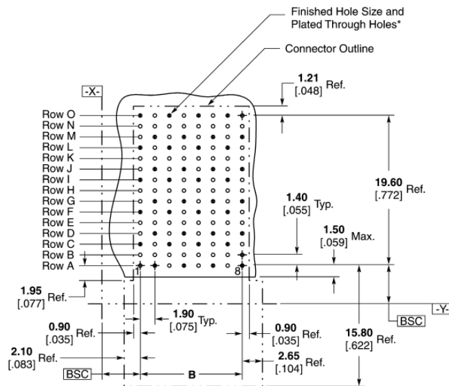
* Finished Hole Diameter = 0.46 \pm^{+0.05}_{-0.002} [018 \pm^{+0.002}_{-0.001} ] Drilled Hole Diameter = 0.55 \pm^{+0.02}_{-0.001} [022 \pm^{+0.001}_{-0.0005} ] Copper Thickness = 0.038 \pm^{+0.013}_{-0.0015} [0015 \pm^{+0.0005}_{-0.0002} ] Tin-Lead Thickness = 0.008 \pm^{+0.004}_{-0.0003} [0003 \pm^{+0.0002}_{-0.0001} ] Finishes other than Tin-Lead. See App. Spec. 114-13202
