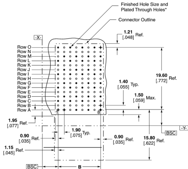
* Finished Hole Diameter = 0.46 \pm^{+0.05}_{-0.002} [018 \pm^{+0.002}_{-0.001} ] Drilled Hole Diameter = 0.55 \pm^{+0.02}_{-0.001} [022 \pm^{+0.001}_{-0.0005} ] Copper Thickness = 0.038 \pm^{+0.013}_{-0.0005} [0015 \pm^{+0.0002}_{-0.0002} ] Tin-Lead Thickness = 0.008 \pm^{+0.004}_{-0.0003} [0003 \pm^{+0.0002}_{-0.0002} ] Finishes other than Tin-Lead. See App. Spec. 114-13202
