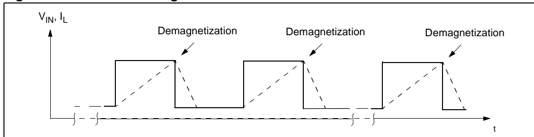
Figure 33. SOT-223 demagnetization
