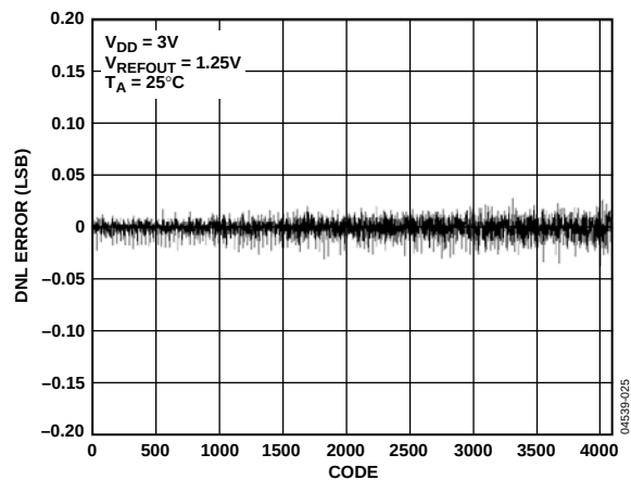
Figure 17. DNL—AD5620-1
