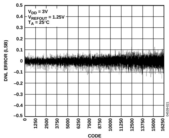
Figure 16. DNL—AD5640-1
