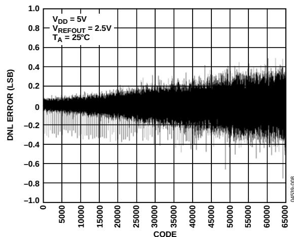
Figure 9. DNL—AD5660-2/AD5660-3
