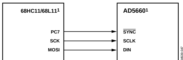
Figure 47. AD5660-to-68HC11/68L11 Interface
