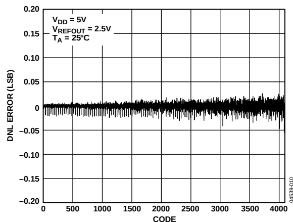
Figure 11. DNL—AD5620-2/AD5620-3
