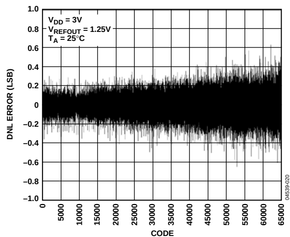
Figure 15. DNL—AD5660-1
