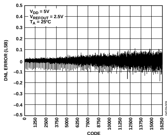
Figure 10. DNL—AD5640-2/AD5640-3
