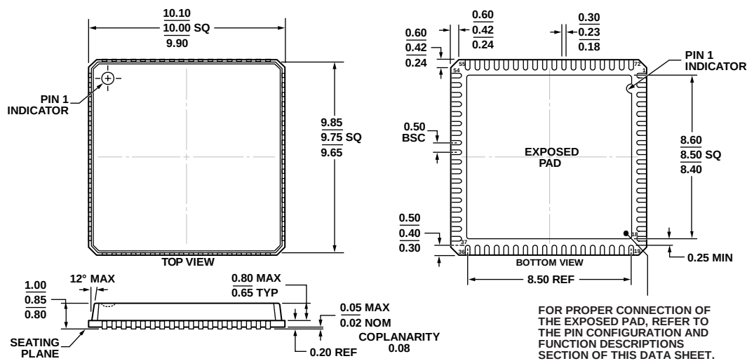
Figure 70. 72-Lead Lead Frame Chip Scale Package, Exposed Pad [LFCSP_VQ] 10 mm x 10 mm Body, Very Thin Quad (CP-72-5) Dimensions shown in millimeters
