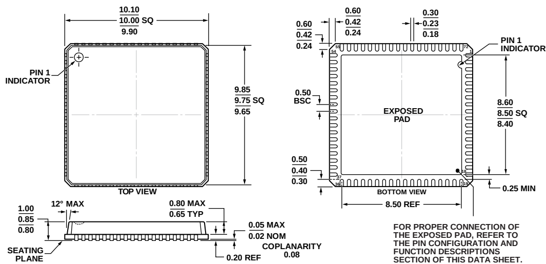
Figure 70. 72-Lead Lead Frame Chip Scale Package, Exposed Pad [LFCSP_VQ] 10 mm × 10 mm Body, Very Thin Quad (CP-72-5)
