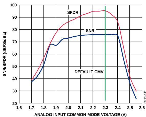
Figure 41. SNR/SFDR vs. Analog Input Common-Mode Voltage, A_{IN} = 100 MHz, 2.5 V p-p FS, AD9467-200
