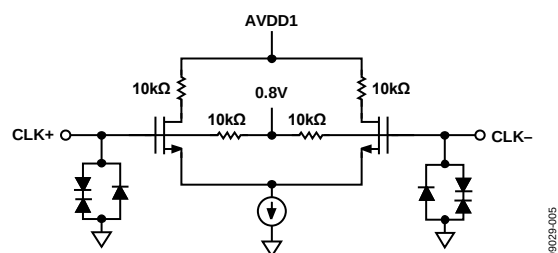
Figure 5. Equivalent Clock Input Circuit
