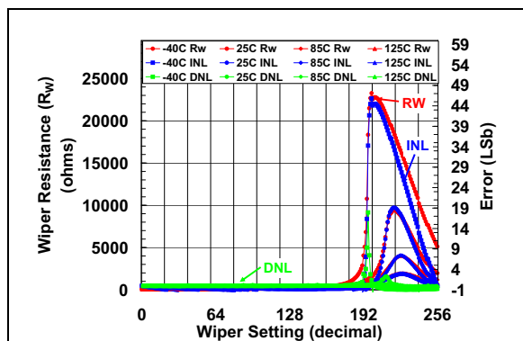
FIGURE 2-70: 100 k \Omega Rheo Mode – R_W ( \Omega ), INL (LSb), DNL (LSb) vs. Wiper Setting and Ambient Temperature ( V_{DD} = 3.0\text{V} ).
