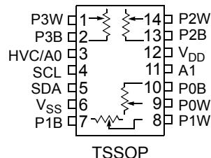
MCP44X2 Quad Rheostat
