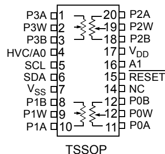
MCP44X1 Quad Potentiometers
