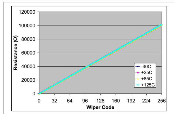
FIGURE 2-74: 100 kΩ – R_{WB} ( \Omega ) vs. Wiper Setting and Ambient Temperature ( V_{DD} = 3.0\text{V} , I_W = 24\ \mu\text{A} ).
