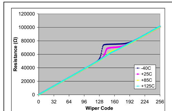
FIGURE 2-74: 100 kΩ – R_{WB} ( \Omega ) vs. Wiper Setting and Ambient Temperature ( V_{DD} = 3.0\text{V} , I_W = 24\ \mu\text{A} ).
