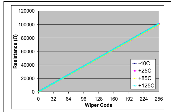
FIGURE 2-73: 100 kΩ – R_{WB} ( \Omega ) vs. Wiper Setting and Ambient Temperature ( V_{DD} = 5.5\text{V} , I_W = 45\ \mu\text{A} ).
