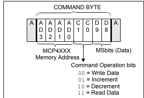
FIGURE 7-1: Command Byte Format.
