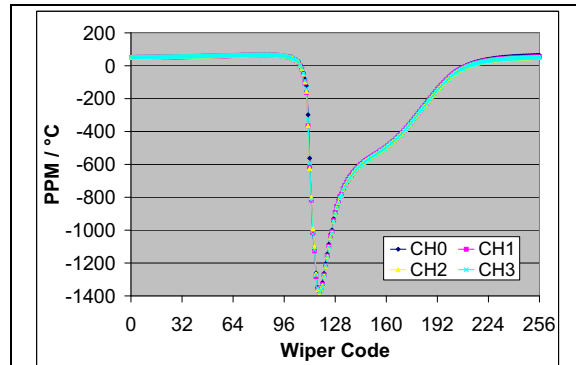
FIGURE 2-40: 10 kΩ – R_{BW} PPM/ ^\circ\text{C} vs. Wiper Setting. ( R_{BW(\text{code}=n, 125^\circ\text{C})} - R_{BW(\text{code}=n, -40^\circ\text{C})} / R_{BW(\text{code}=256, 25^\circ\text{C})} / 165^\circ\text{C} * 1,000,000 ) ( V_{DD} = 3.0\text{V} , I_W = 150\text{ }\mu\text{A} ).
