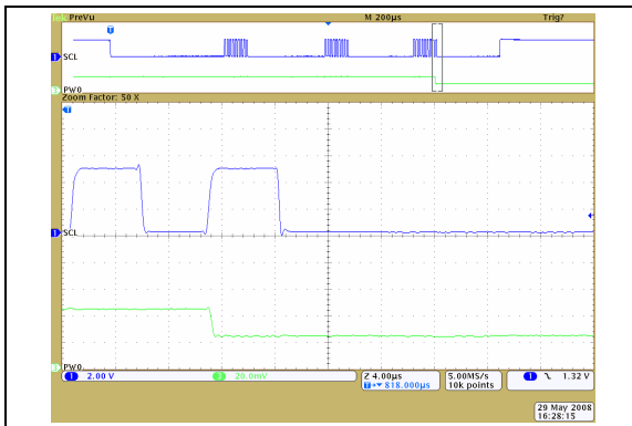
FIGURE 2-43: 10\text{ k}\Omega – Low-Voltage Decrement Wiper Settling Time ( V_{DD} = 5.5\text{V} ) ( 1\text{ }\mu\text{s}/\text{Div} ).
