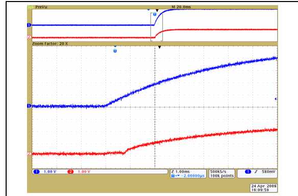
FIGURE 2-44: 10\text{ k}\Omega – Low-Voltage Increment Wiper Settling Time ( V_{DD} = 2.7\text{V} ) ( 1\text{ }\mu\text{s}/\text{Div} ).
