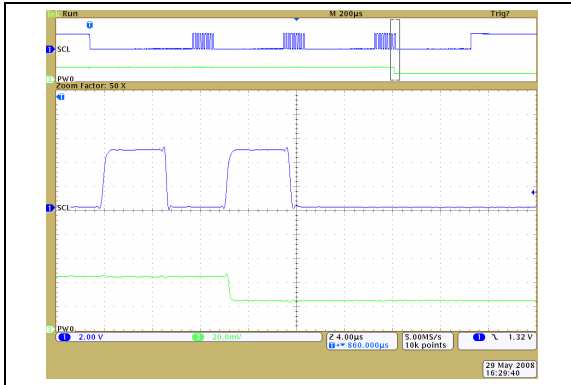
FIGURE 2-42: 10\text{ k}\Omega – Low-Voltage Decrement Wiper Settling Time ( V_{DD} = 2.7\text{V} ) ( 1\text{ }\mu\text{s}/\text{Div} ).
