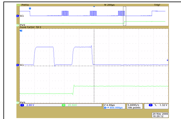
FIGURE 2-45: 10\text{ k}\Omega – Low-Voltage Increment Wiper Settling Time ( V_{DD} = 5.5\text{V} ) ( 1\text{ }\mu\text{s}/\text{Div} ).
