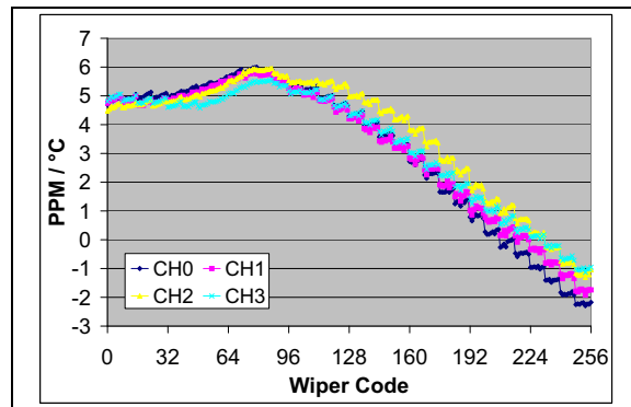
FIGURE 2-59: 50 kΩ – R_{WB} PPM/°C vs. Wiper Setting. ( R_{BW(\text{code}=n, 125^\circ\text{C})} - R_{BW(\text{code}=n, -40^\circ\text{C})} / R_{BW(\text{code}=256, 25^\circ\text{C})} / 165^\circ\text{C} * 1,000,000 ) ( V_{DD} = 5.5\text{V} , I_W = 90\text{ }\mu\text{A} ).
