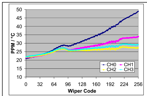
FIGURE 2-39: 10 kΩ – R_{BW} PPM/°C vs. Wiper Setting. ( R_{BW(\text{code}=n, 125^\circ\text{C})} - R_{BW(\text{code}=n, -40^\circ\text{C})} / R_{BW(\text{code}=256, 25^\circ\text{C})} / 165^\circ\text{C} * 1,000,000 ) ( V_{DD} = 5.5\text{V} , I_W = 150\text{ }\mu\text{A} ).
